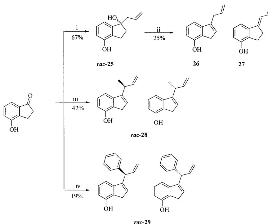
Scheme 4. (i) Allyl bromide, Zn, \text{NH}_4\text{Cl}_{\text{aq}} /THF. (ii) \text{MgSO}_4 , toluene, reflux. (iii) Crotyl bromide, Zn, \text{NH}_4\text{Cl}_{\text{aq}} /THF. (iv) Cinnamyl chloride, Zn, \text{NH}_4\text{Cl}_{\text{aq}} /THF.
