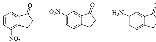
Figure 1. Nitro- and amino-substituted 1-indanones yielding no reaction with crotyl bromide/Zn and crotyl bromide/In.
