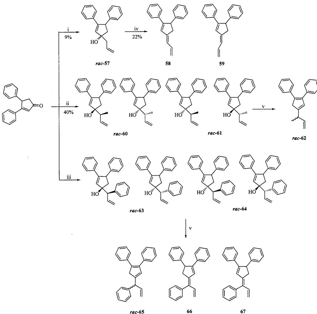
Scheme 10. (i) Allyl bromide, Zn, \text{NH}_4\text{Cl}_{\text{aq}} /THF. (ii) Crotyl bromide, Zn, \text{NH}_4\text{Cl}_{\text{aq}} /THF. (iii) Cinnamyl chloride, Zn, \text{NH}_4\text{Cl}_{\text{aq}} /THF. (iv) Amberlyst 15, pentane. (v) \text{MgSO}_4 , toluene, reflux.
