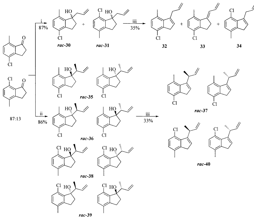
Scheme 5. (i) Allyl bromide, Zn, \text{NH}_4\text{Cl}_{\text{aq}} /THF. (ii) Crotyl bromide, Zn, \text{NH}_4\text{Cl}_{\text{aq}} /THF. (iii) Amberlyst 15, pentane.
