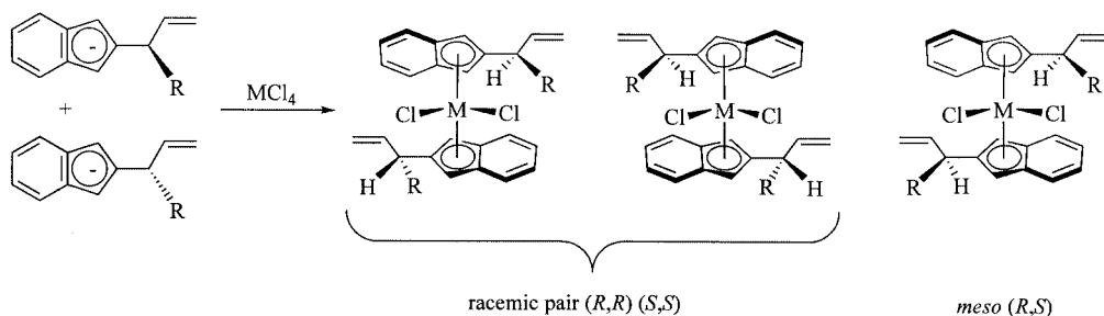
Scheme 15. Metallation of 2-substituted indenyls.
