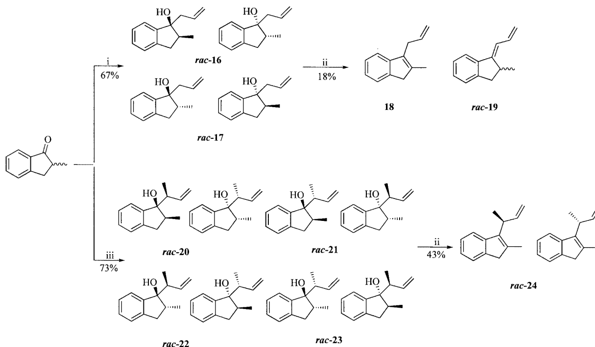
Scheme 3. (i) Allyl bromide, Zn, \text{NH}_4\text{Cl}_{\text{aq}} /THF. (ii) Amberlyst 15, pentane. (iii) Crotyl bromide, Zn, \text{NH}_4\text{Cl}_{\text{aq}} /THF.
