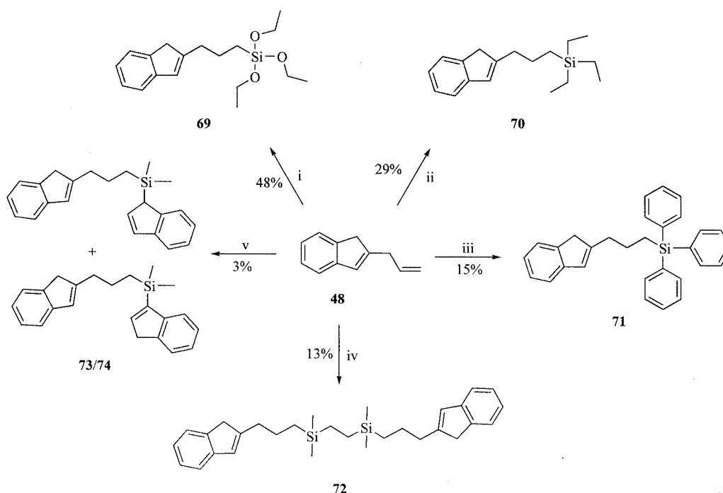
Scheme 12. Karstedt's catalyst in toluene with (i) triethoxysilane, (ii) triethylsilane, (iii) triphenylsilane, (iv) 1,2-bis(dimethylsilyl)ethane, and (v) (1H-inden-1-yl)dimethylsilane (containing about 10% of (3H-inden-1-yl)dimethylsilane as impurity).
