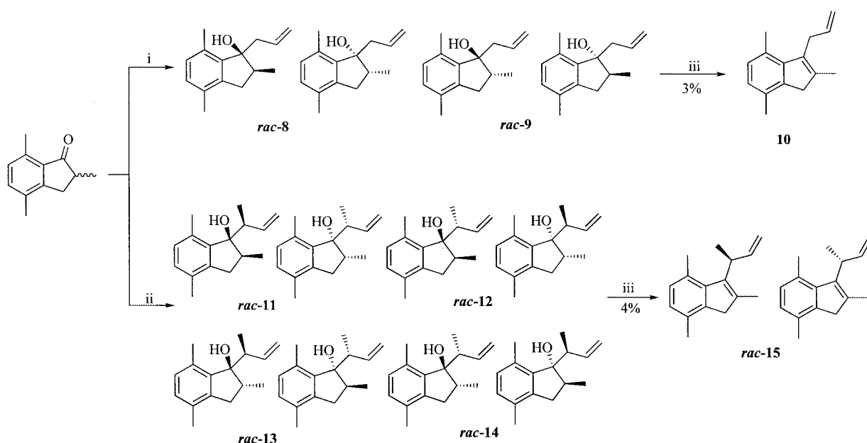
Scheme 2. (i) Allyl bromide, Zn, NH 4 Cl aq /THF. (ii) Crotyl bromide, Zn, NH 4 Cl aq /THF. (iii) Amberlyst 15, pentane.
