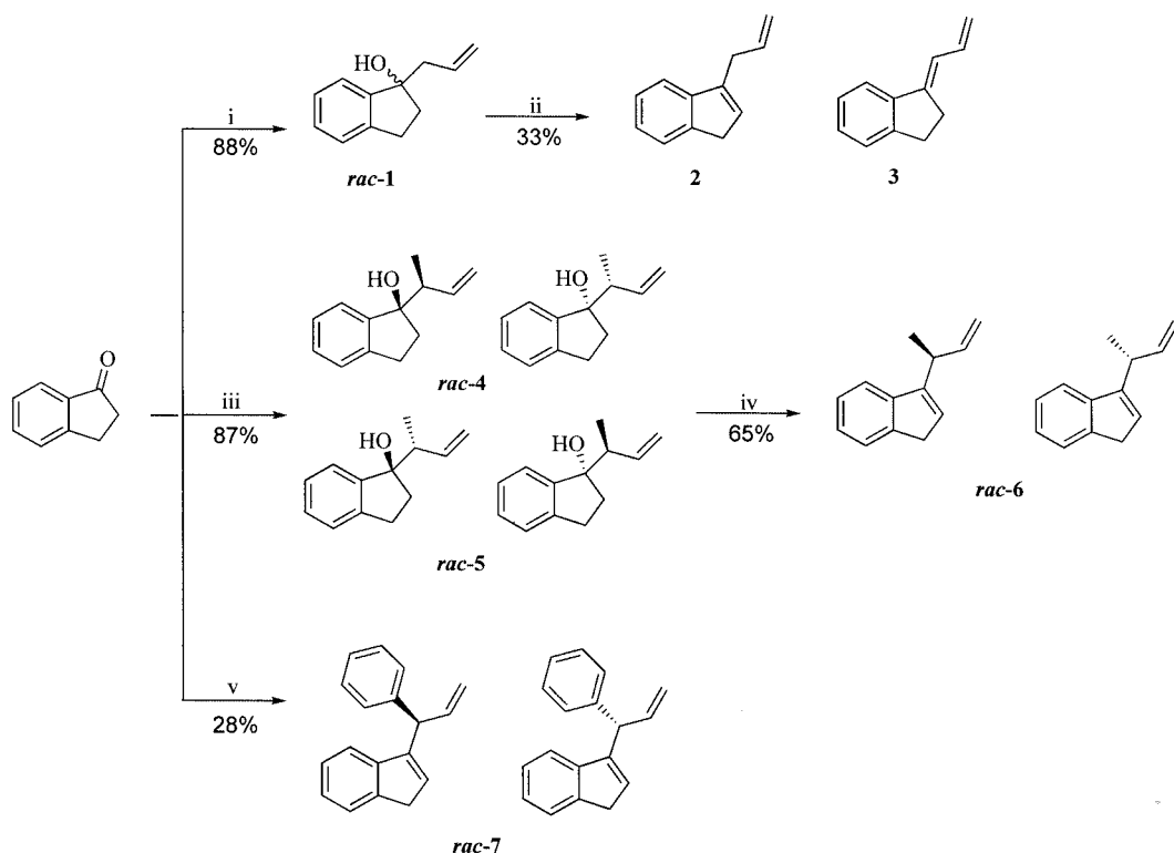
Scheme 1. (i) Allyl bromide, Zn, NH 4 Cl aq /THF. (ii) Amberlyst 15, pentane. (iii) Crotyl bromide, Zn, NH 4 Cl aq /THF. (iv) Amberlyst 15, pentane. (v) Cinnamyl chloride, Zn, NH 4 Cl aq /THF.
