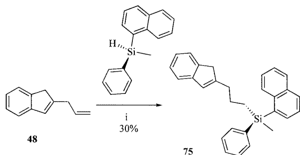
Scheme 13. (i) (+)-( R )-Methyl-1-naphthalenylphenylsilane, Karstedt's catalyst, toluene.
