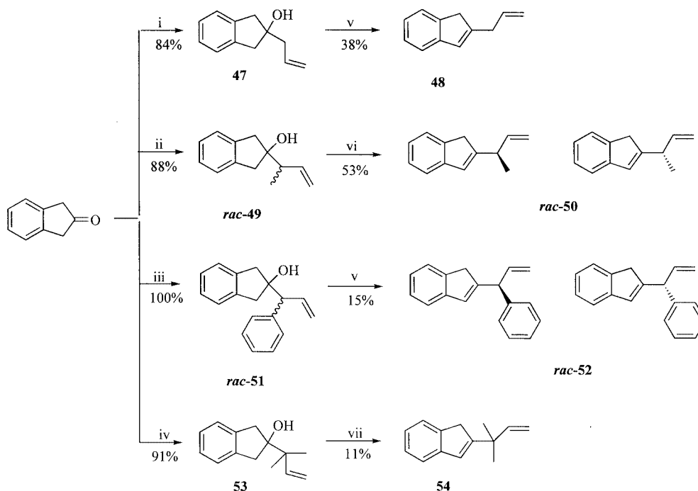
Scheme 8. (i) Allyl bromide, Zn, \text{NH}_4\text{Cl}_{\text{aq}} /THF. (ii) Crotyl bromide, Zn, \text{NH}_4\text{Cl}_{\text{aq}} /THF. (iii) Cinnamyl chloride, Zn, \text{NH}_4\text{Cl}_{\text{aq}} /THF. (iv) Prenyl bromide, Zn, \text{NH}_4\text{Cl}_{\text{aq}} /THF. (v) p -TSA, toluene, reflux. (vi) \text{H}_2\text{SO}_4 , toluene, reflux. (vii) Amberlyst 15, pentane.
