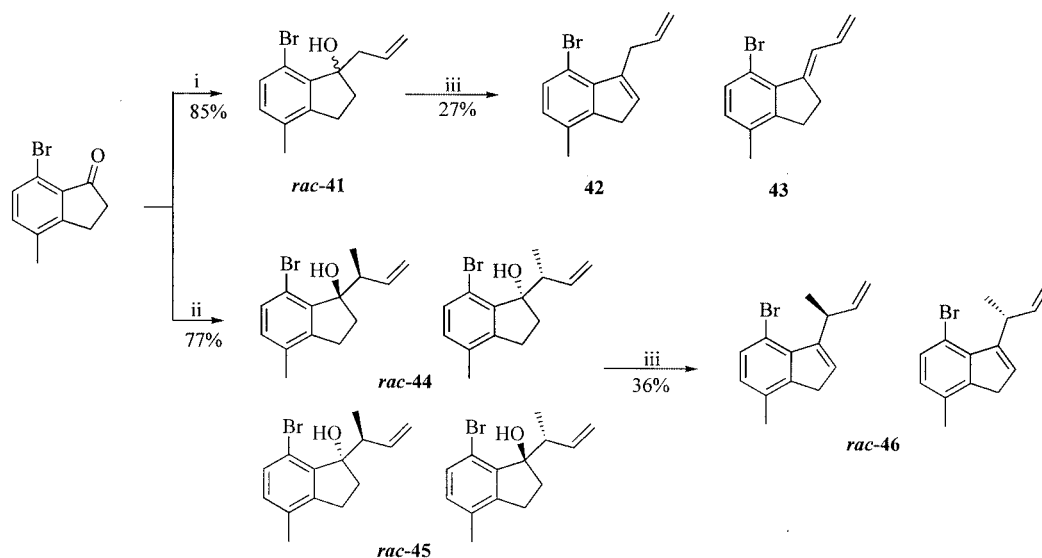
Scheme 6. (i) Allyl bromide, Zn, \text{NH}_4\text{Cl}_{\text{aq}} /THF. (ii) Crotyl bromide, Zn, \text{NH}_4\text{Cl}_{\text{aq}} /THF. (iii) Amberlyst 15, pentane.
