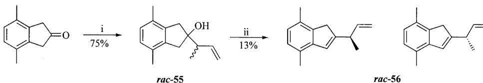
Scheme 9. (i) Crotyl bromide, Zn, \text{NH}_4\text{Cl}_{\text{aq}} /THF. (ii) Amberlyst 15, pentane.
