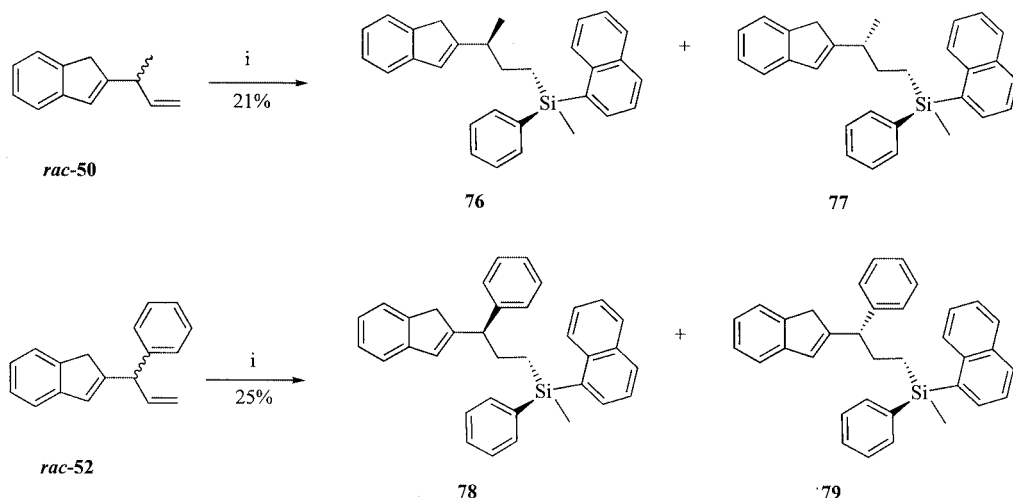
Scheme 14. (i) (+)-( R )-Methyl-1-naphthalenylphenylsilane, Karstedt's catalyst, toluene.
