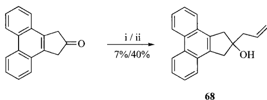
Scheme 11. i) Allyl bromide, Zn, NH 4 Cl/THF. (ii) Allyl bromide, In, water/THF.
